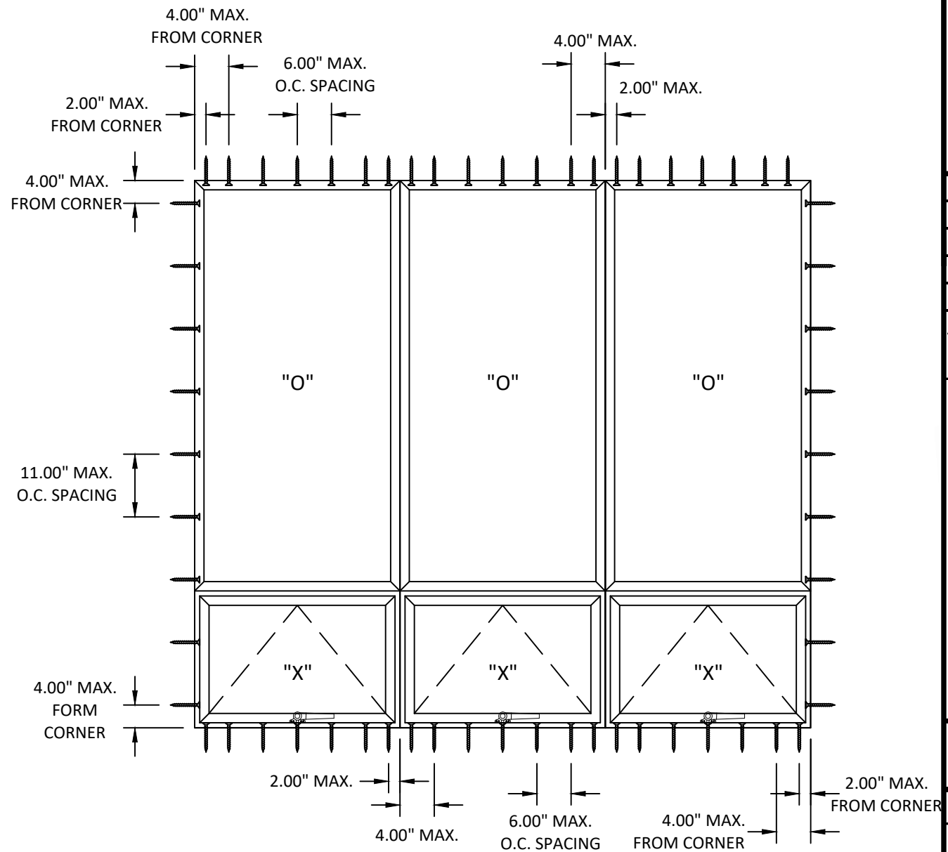
TYPICAL ANCHOR LAYOUT THROUGH FRAME
