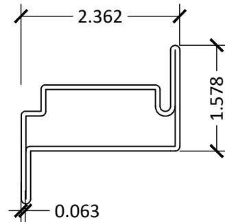
13 DOOR STILE
