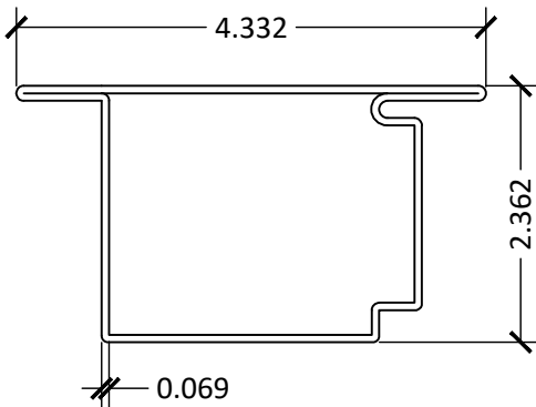
12 MULLION
